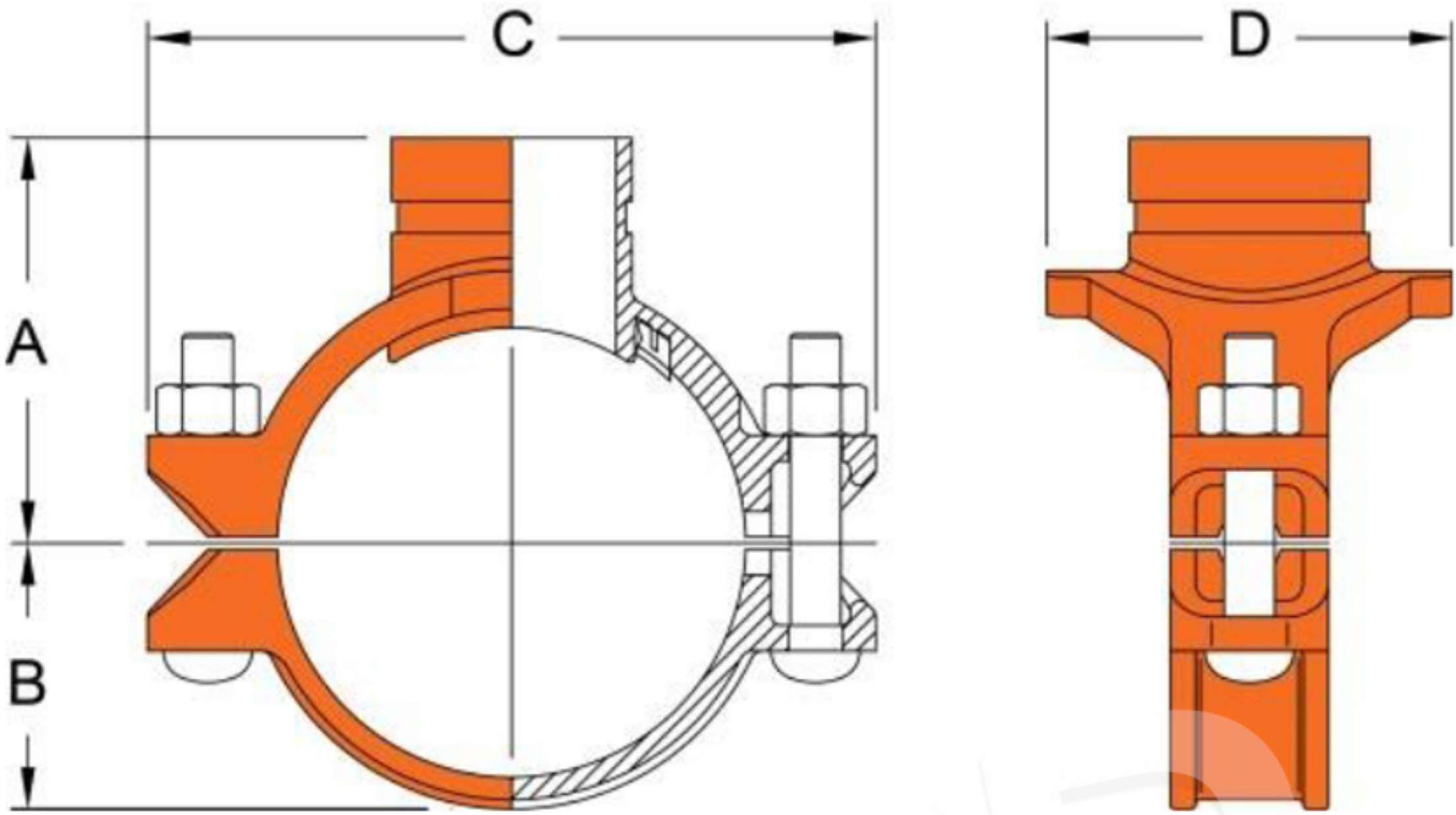
Model 7722 Mechanical Tee, Grooved-End Outlet
